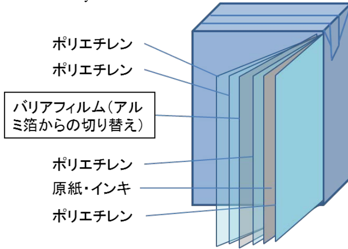
Figure 1: Constituent Layers of the FUJIPAK
