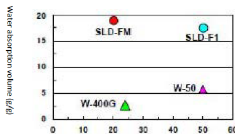
Comparison between powdered cellulose and Sunrose® SLD for average particle size and water absorption
